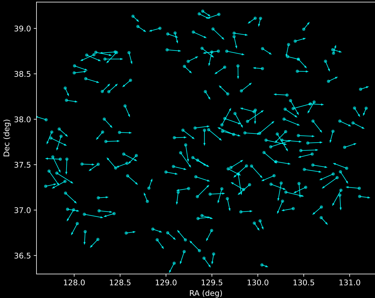
APOGEE DR17 Noise Stream Proper Motion Vectors (n=187)
