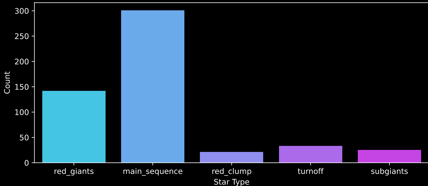
APOGEE DR17 Field: [N752_btx] Count plot of Star Type
