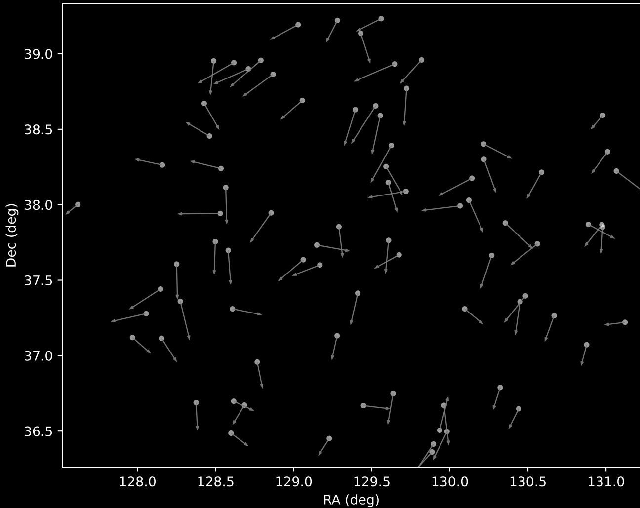
APOGEE DR17 Cluster 14 Proper Motion Vectors (n=81)
