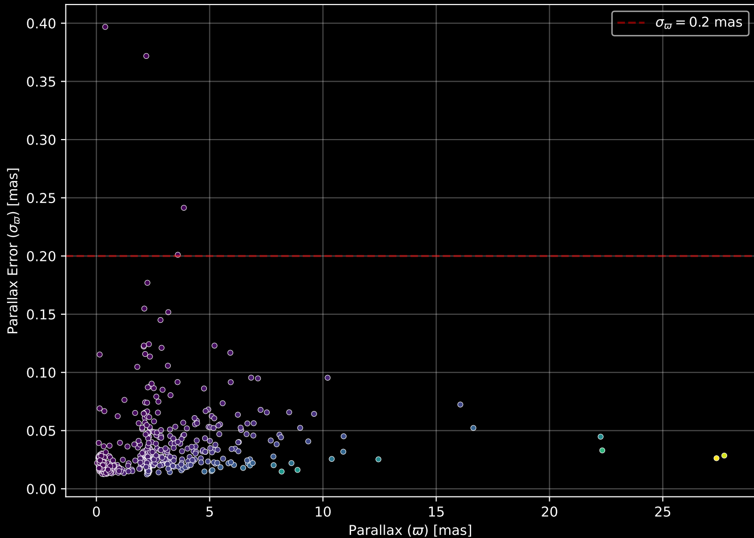
APOGEE DR17 Field: [N752_btx] Parallax Quality (n= 522)
