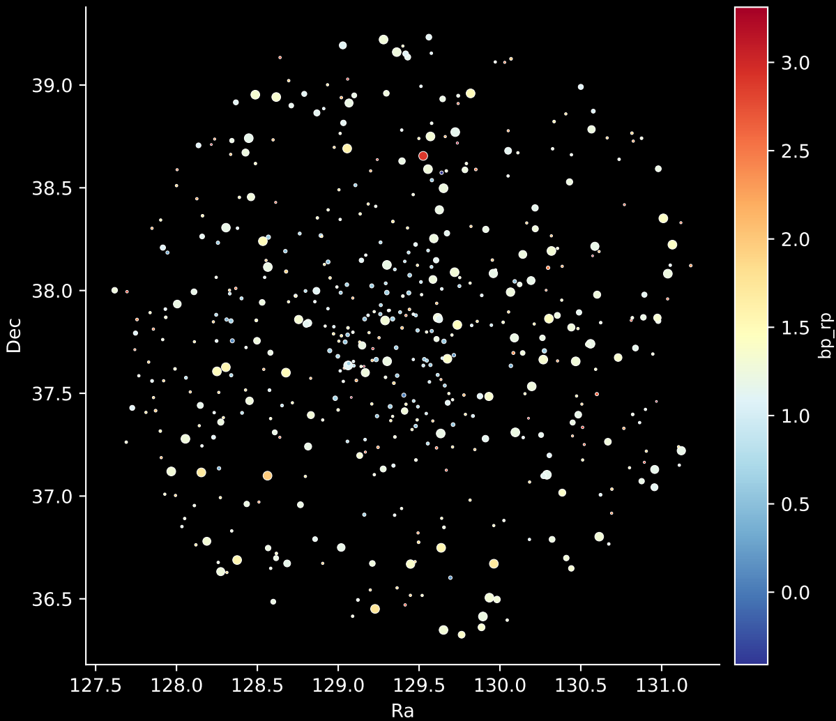
APOGEE DR17 Field: [N752_btx] Stars: 522
