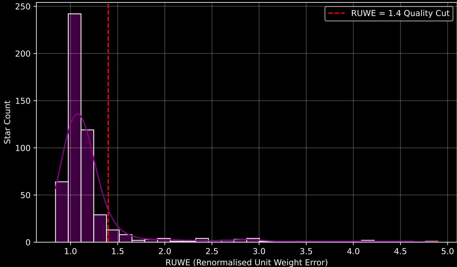
GAPOGEE DR17 Field [N752_btx] RUWE Distribution (n= 511)
