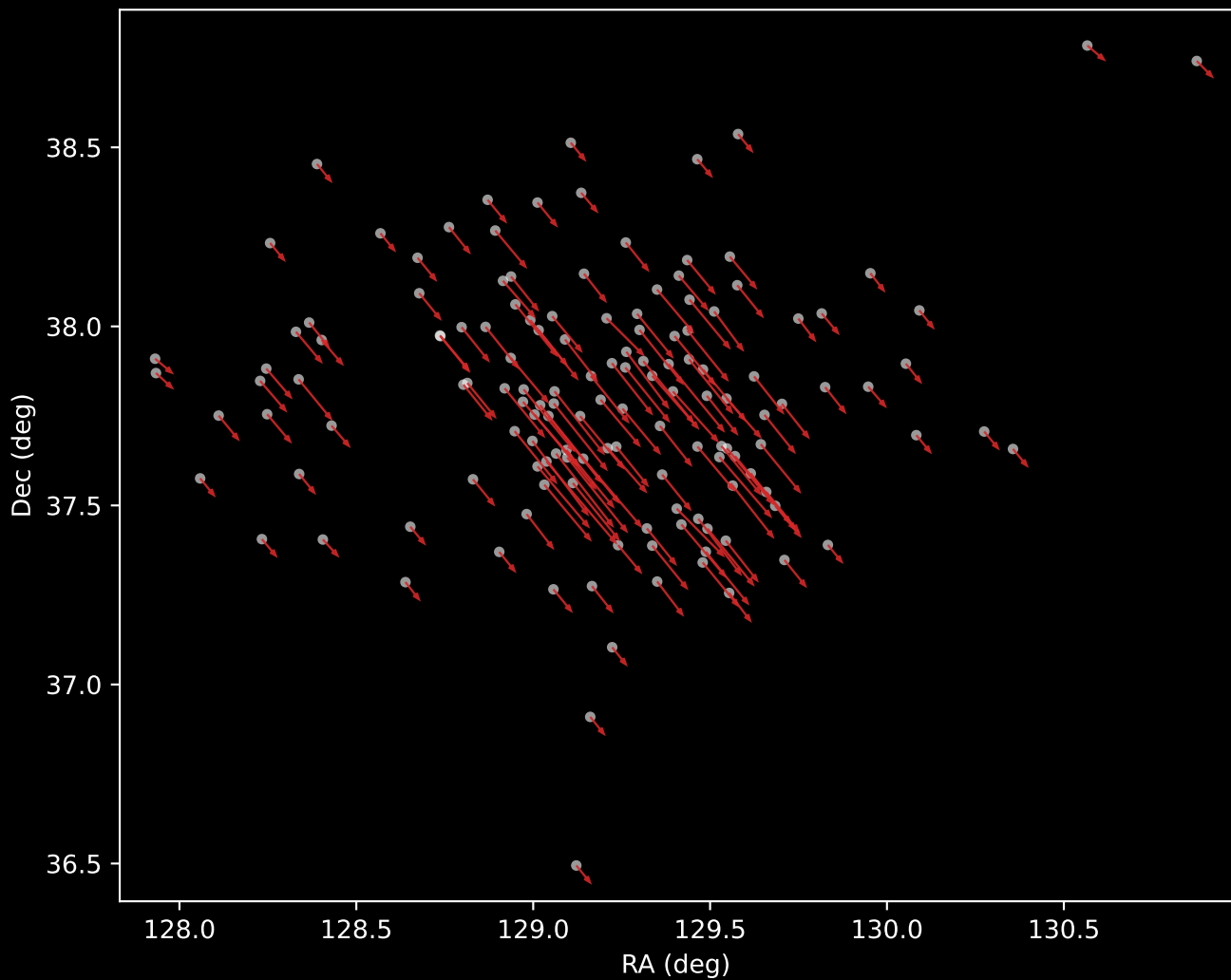
APOGEE DR17 Cluster 6 Proper Motion Vectors (n=142)
