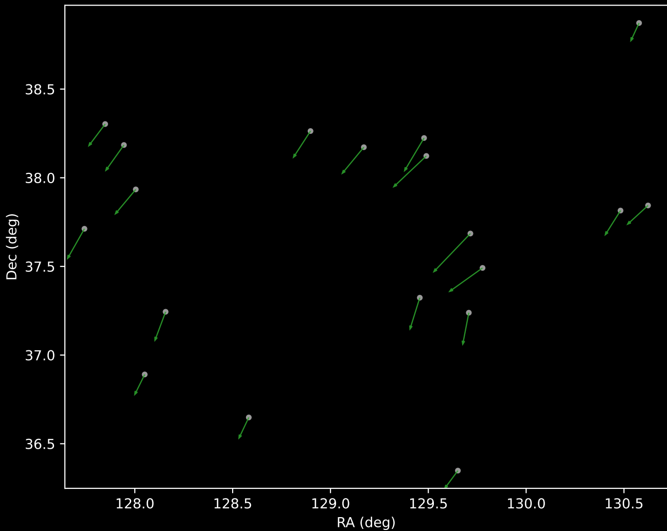
APOGEE DR17 Cluster 4 Proper Motion Vectors (n=19)
