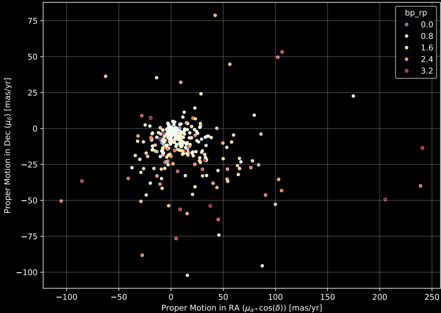
APOGEE DR17 Field: [N752_btx] Proper Motion Diagram (n= 522)
