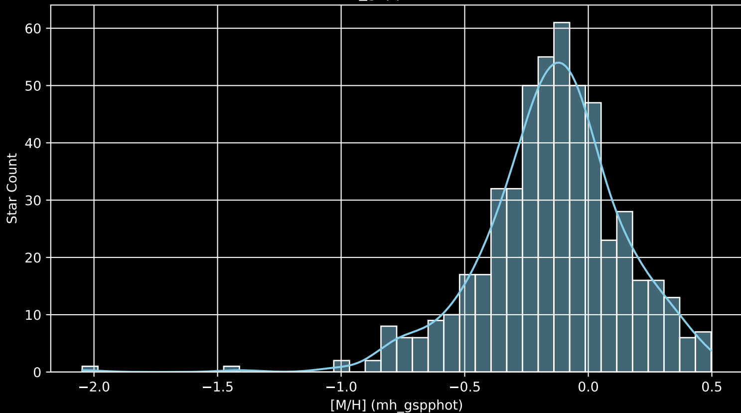
APOGEE DR17 Field: [N752_btx [M/H] (mh_gspphot) (n= 515)
